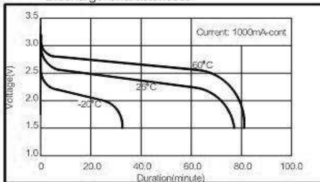
Discharge Characteristics
